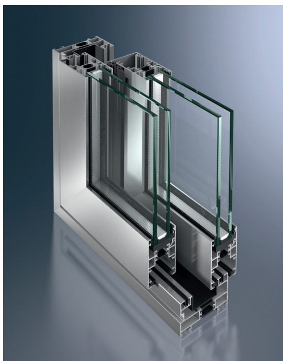
Schüco ASS 48, sistem glisant izolat termic Schüco ASS 48, thermally insulated sliding system
