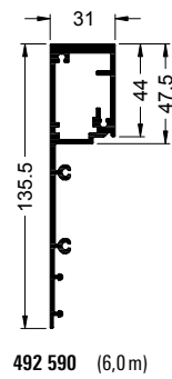
Verhakungsprofil, Standard Interlock profile, standard
